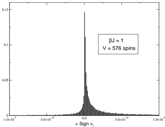
FIG. 2: Probability distribution of \langle \text{Sign} \rangle_i for the kagomé lattice with V = 576 spins and \beta J = 1 .
