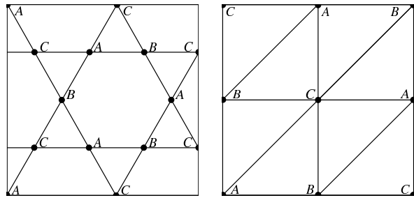
FIG. 1: kagomé lattice (left) and frustrated square (or anisotropic triangular) lattice (right) consisting of three sub-lattices A, B, C.
