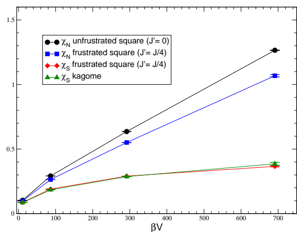
FIG. 4: Coplanar staggered susceptibility \chi_s and collinear Néel susceptibility \chi_N as functions of the space-time volume \beta V for the kagomé as well as the frustrated ( J' = J/4 ) and unfrustrated ( J' = 0 ) square lattice at fixed space/time aspect ratio \sqrt{V}/\beta J = 20 .
