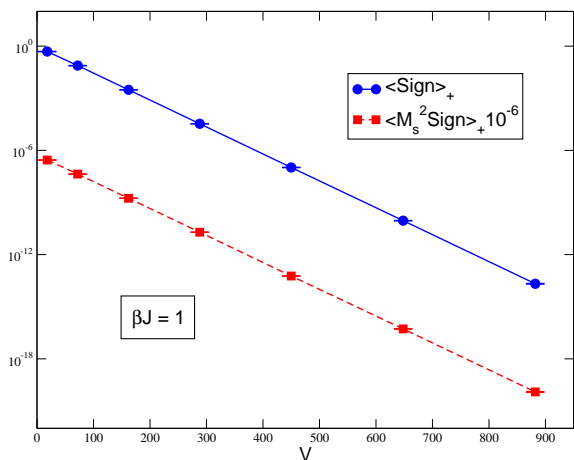
FIG. 3: Volume-dependence of \langle \text{Sign} \rangle_+ and \langle M_s^2 \text{Sign} \rangle_+ (rescaled by 10^{-6} ) for the kagomé lattice with \beta J = 1 .
